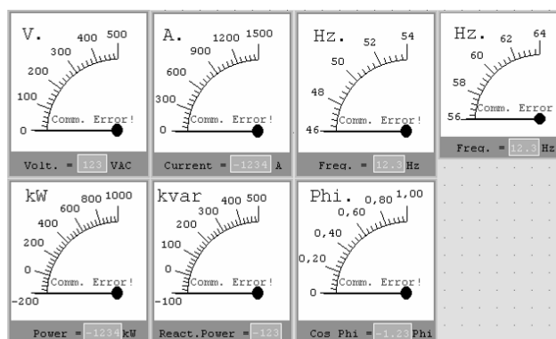
Figure 4 - 90 degrees DeifMeters
