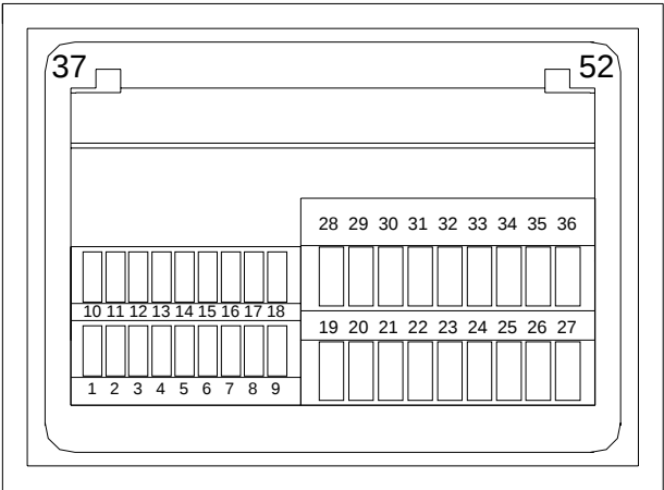
Rear view of EC-1
