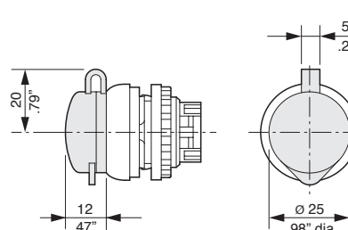
Protection cap P SN/XWS
