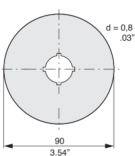
Emergency stop plates P SN/XAK
