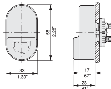
Protection cap P SN/T/DD
