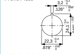
With single hole mounting 22 mm
